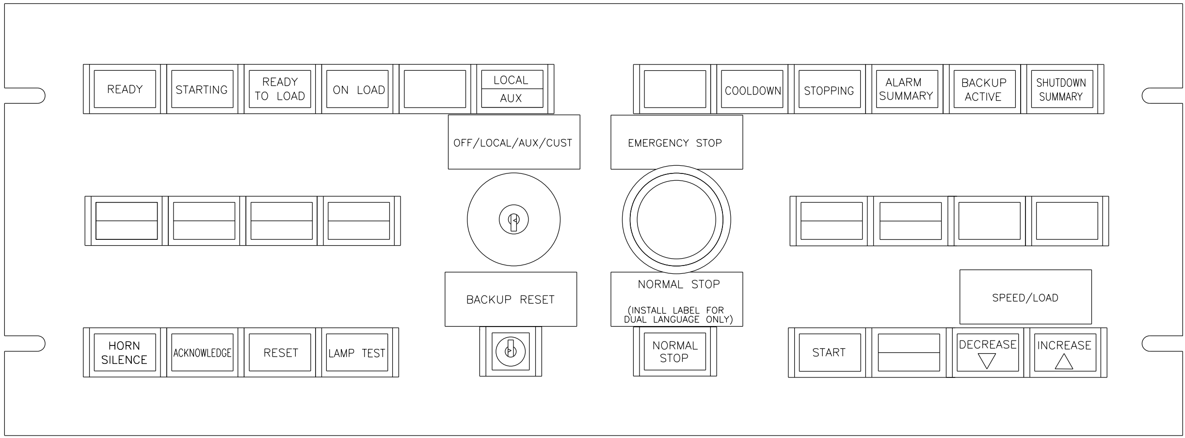
FRONT VIEW
