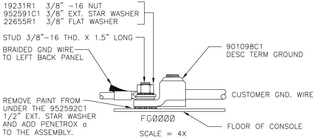
TYPICAL GROUND STUD ASSEMBLY
